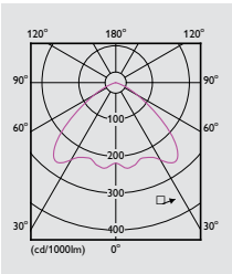
HPK518 1xHPI-P250W BU WB Alu Reflector with PG-IP65
