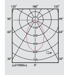
HPK518 1xHPL-N250W NB Alu Reflector with PG-IP65
