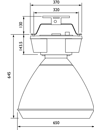
Prismatic Reflector + Cover Lens
