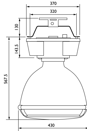
Aluminium Reflector + Thermoplastic Cover
