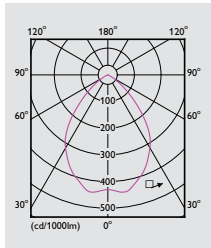
HPK518 1xHPI-P250W BU NB Alu Reflector with PG-IP65
